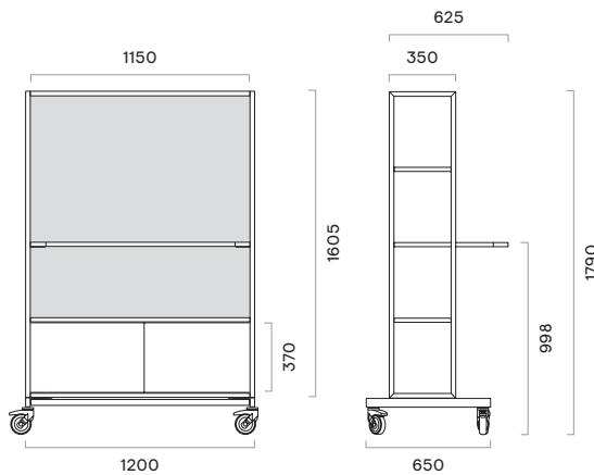
Mobile workstation with fixed cabinet and back panel
